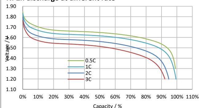
Ni-Zn discharge at different rate
